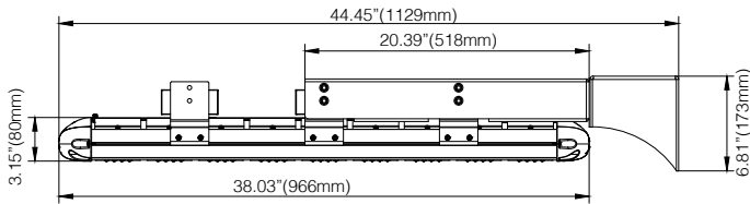
AR-XAL WITH STRAIGHT ARM
