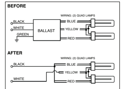
Figure 4: Retrofit with two lamps (G24q Base)
