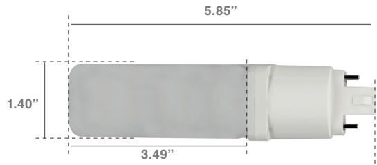
12W Horizontal
