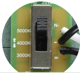
Internal CCT Selectable Switch
