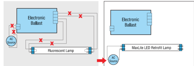
Figure 2. Single sided connection
